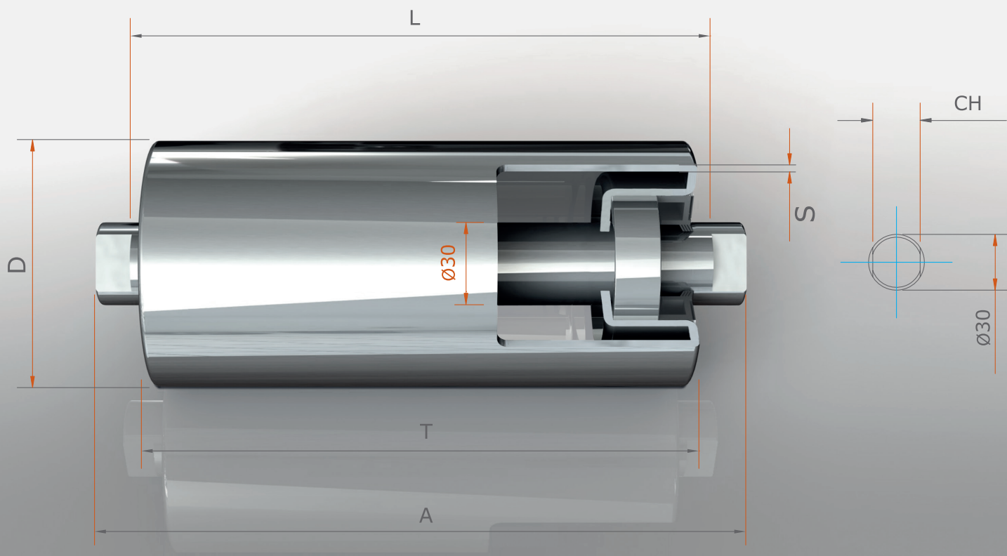
RULLI FOLLI P600 - P600 IDLER ROLLERS
