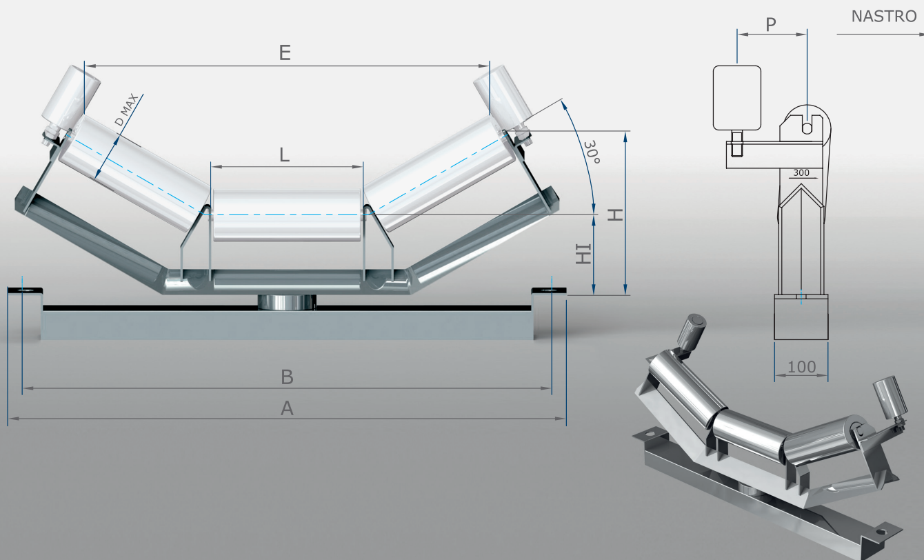
30° AUTOCENTRANTI IN ANGOLARE - 30° ANGLE BAR SELF-CENTRING ELEMENTS
